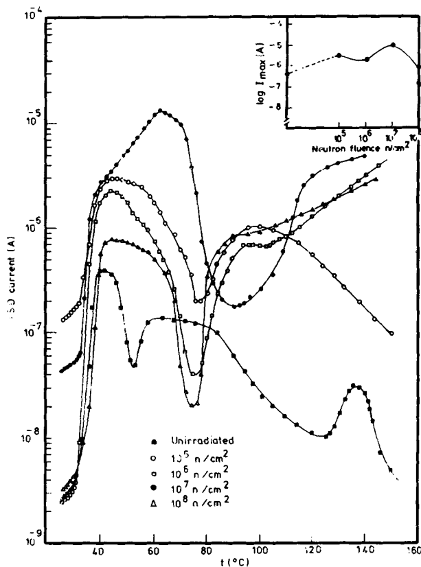
Figure 7 Temperature dependence of TSDC for doped PVA with 40 wt % NiCl 2 of different neutron fluences.
