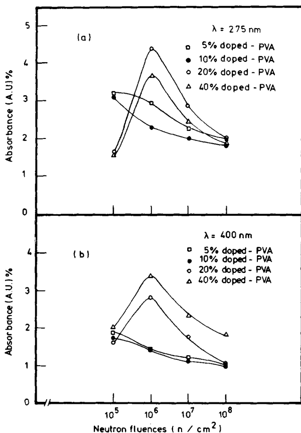
Figure 2 Variation of absorbance as a function of neutron fluences at (a) \lambda = 275 nm and (b) \lambda = 400 nm for NiCl 2 -doped PVA specimens.
