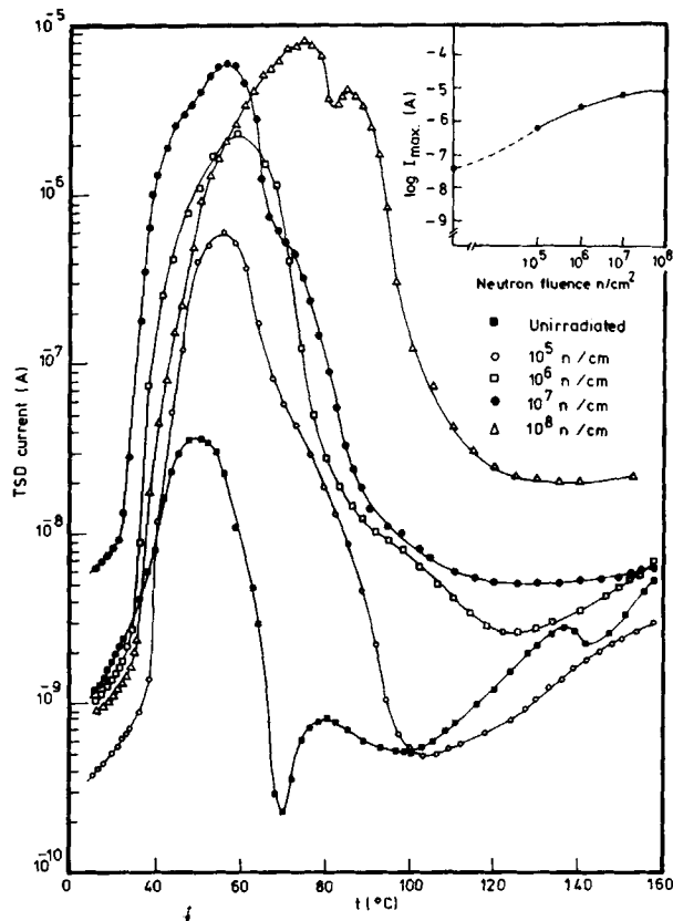
Figure 4 Temperature dependence of TSDC doped PVA with 5 wt % \text{NiCl}_2 at different neutron fluences.
